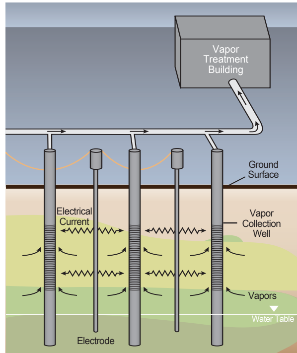
Example of an in situ thermal treatment system.
